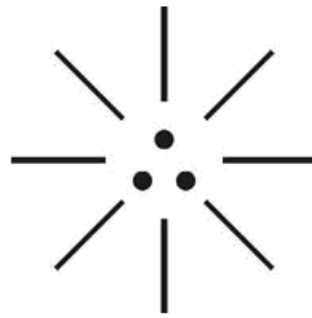
(ALL-E)
